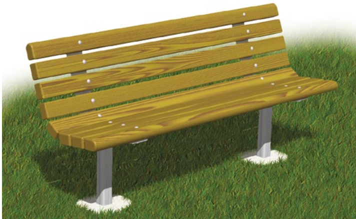
Model SWRB/G-6TP 6 Ft. Embedded Mount Bench with Hot Dip Galvanized Frames and Pressure Treated Southern Yellow Pine 3" x 4" timbers.
